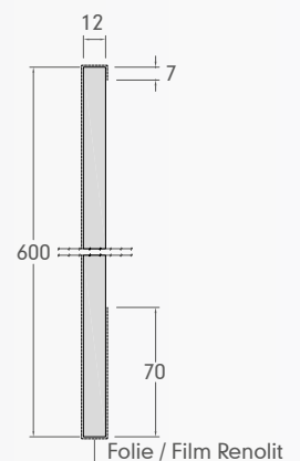
RLK 600 (3660 mm) ral 9016/9001/9001 HN*
