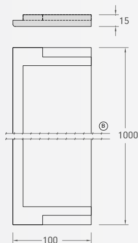
RLK E 03 (1000 mm) ral 9016/9001/9001 HN*
