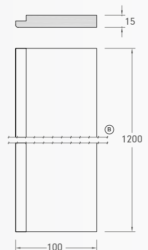
RLK E 05 (1200 mm) ral 9016/9001/9001 HN*
